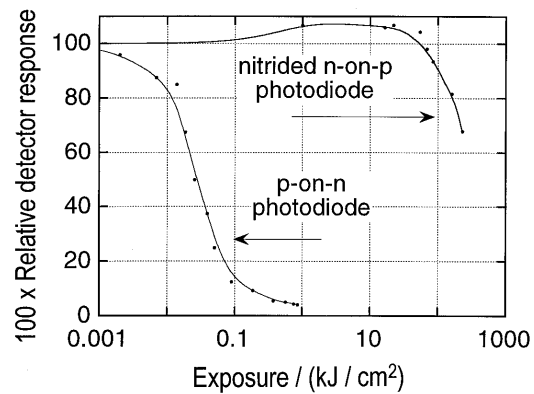
Figure 6. The degradation of one of the n-on-p silicon photodiodes during prolonged exposure to a pulsed laser at \lambda=193 nm. Also plotted is the corresponding degradation of a p-on-n silicon photodiode.
